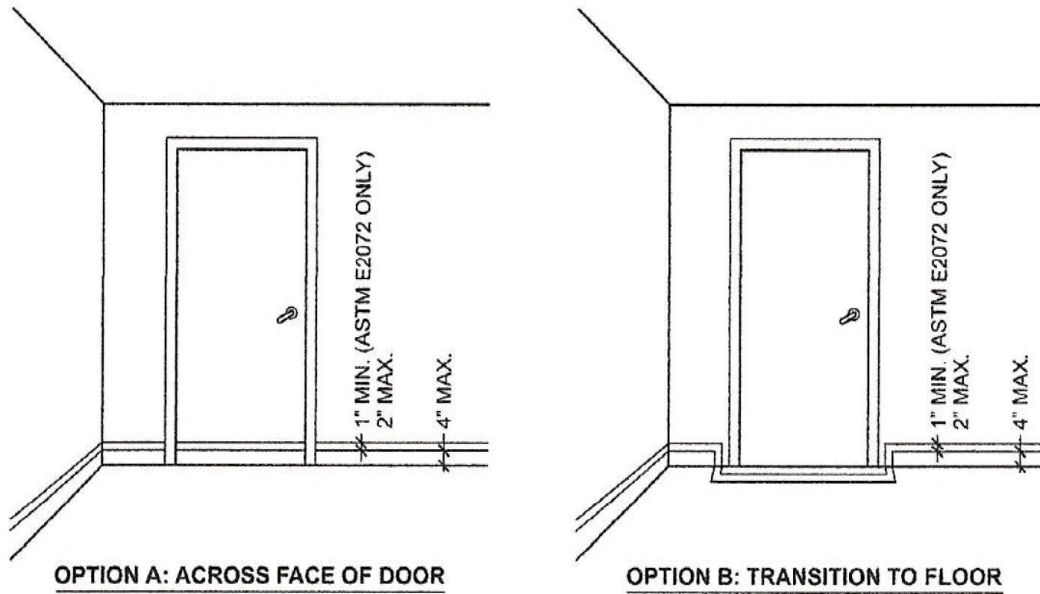
FIGURE S101.1(8) WALL-MOUNTING OPTION FOR PHOTOLUMINESCENT PERIMETER DEMARCATION LINES THAT ARE NOT PROVIDED WITH DOOR FRAME MARKING
